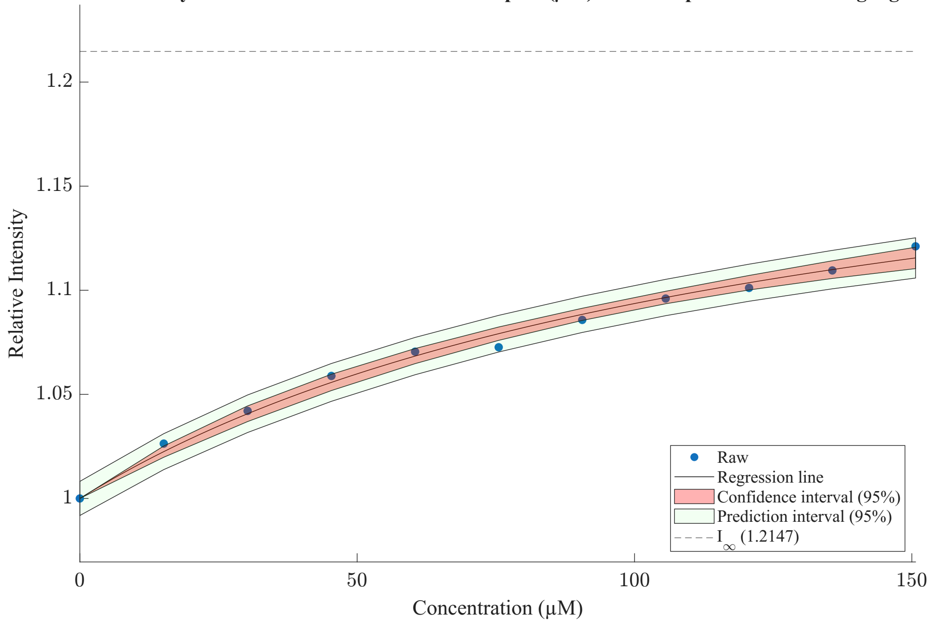
Relative intensity as a function of concentration of lipids (μM) for a6r rep2 - Statistics fitting algorithm
